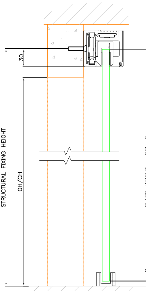
SECTION A-A FULL GLASS LEAF Scale, 1:2,5
