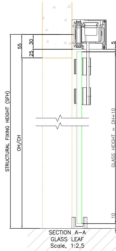
SECTION A-A GLASS LEAF
