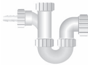
OPP-ZB35068DB P Trap Tee 76 mm Seal - 40 mm
