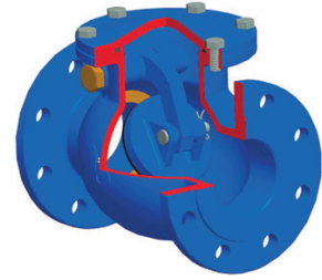
BRD-S6-100 Swing Check Valve Available in Sizes from - DN40 - DN800
