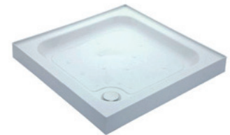
BDJ-A80100-WH Stone Resin/Acrylic Capped Shower Tray 50 mm Waste 800 x 800 x 130 mm
