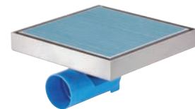
Stainless Steel Tile Drain Universal Outlet Dia. 50 mm Capacity - 35 l/m
