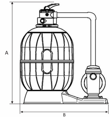
"AQUARIUS" Filtration System
