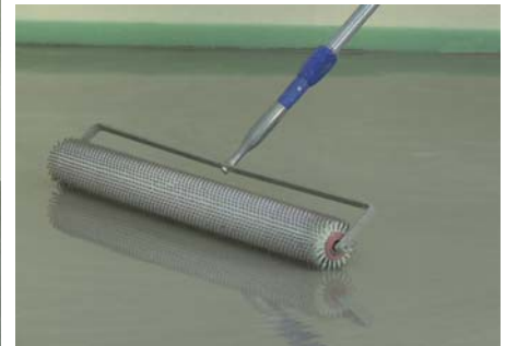
Removing residual pores with a needle roller
