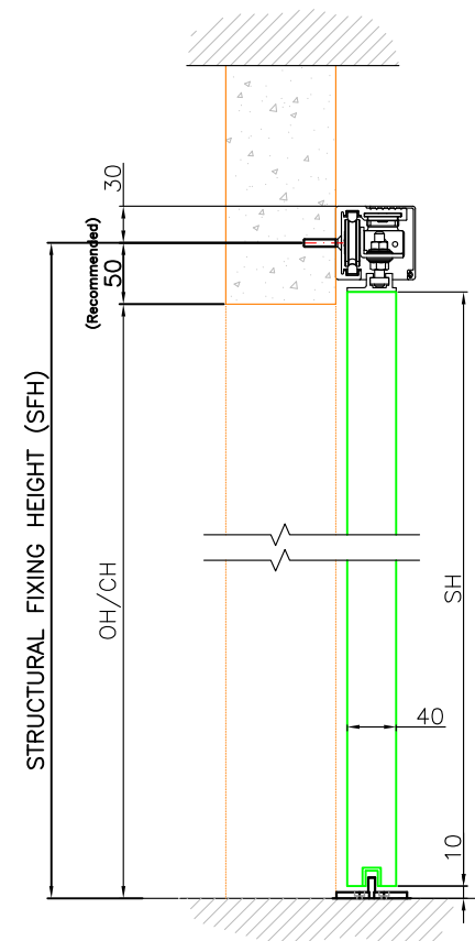
SECTION A-A TIMBER LEAF Scale, 1:5
