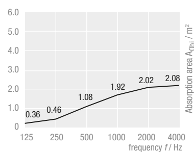
THERMATEX® Sonic element round Ø 1200 mm, Assembly height 300 mm
