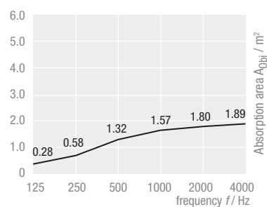
THERMATEX® Sonic element round Ø 1200 mm, Assembly height 150 mm
