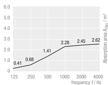
THERMATEX® Sonic element square 1200 x 1200 mm, Assembly height 300 mm
