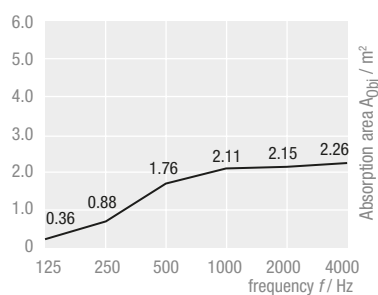
THERMATEX® Sonic element square 1200 x 1200 mm, Assembly height 150 mm
