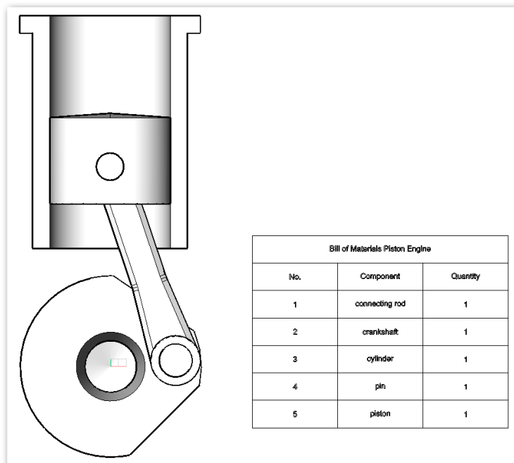
BOM table inserted in a drawing
