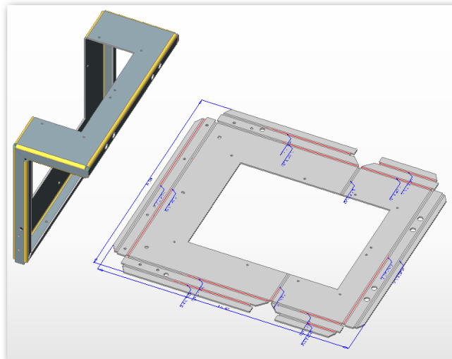
3D model flattened, ready for export to CNC machinery
