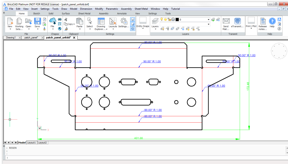
Sheet metal part unfolded and automatically dimensioned
