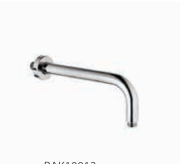
RAK10012 Shower ARM (250 mm ) D15 1/2" Male Thread with sliding Cover Plate
