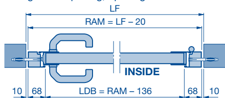
Fitting behind the opening
