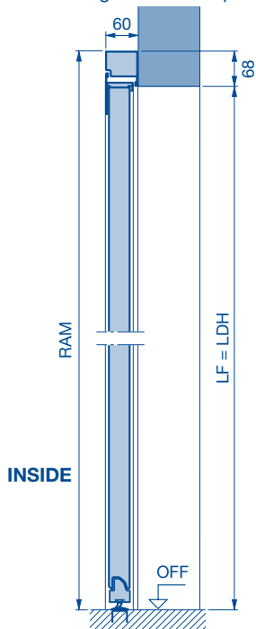
Fitting behind the opening
