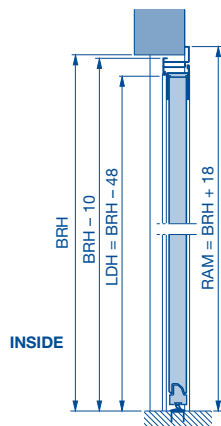
External fitting
