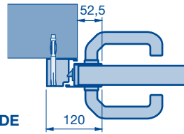
Profile type 2 Wide leaf frame
