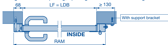
Fitting behind the opening, opening inwards, RH or LH hinged
