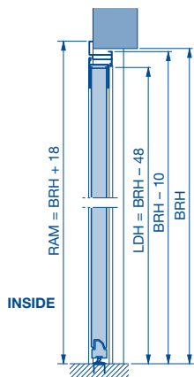
Internal fitting
