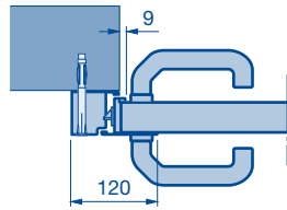
Profile type 1 Narrow leaf frame
