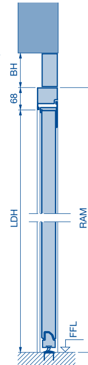
Panel over the side door
