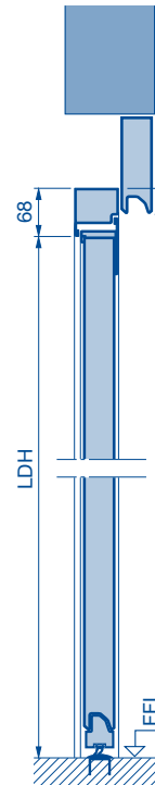
Panel in front of the side door
