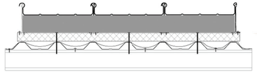
SUPERSEAM Standing Seam System
