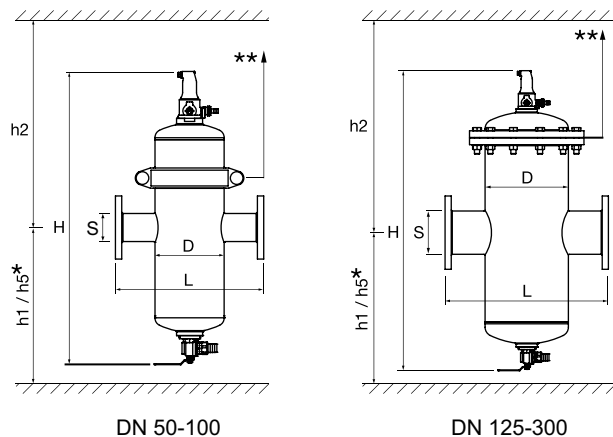
Zeparo ZEK...F Extended type. Flange connection PN 16. Horizontal installation.
