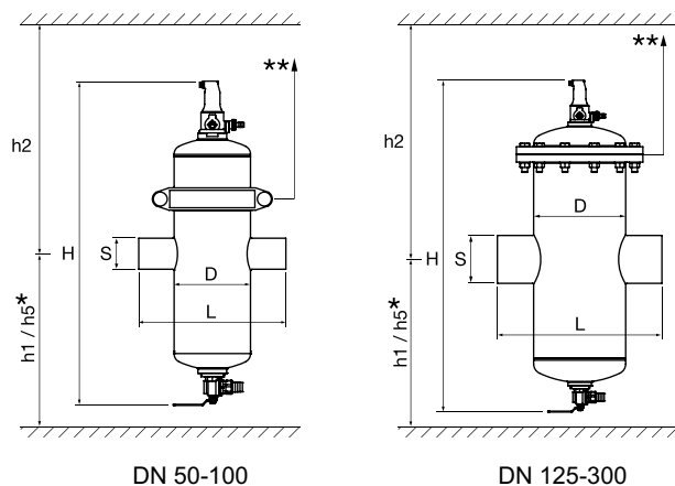
Zeparo ZEK...S Extended type. Welding connection. Horizontal installation.
